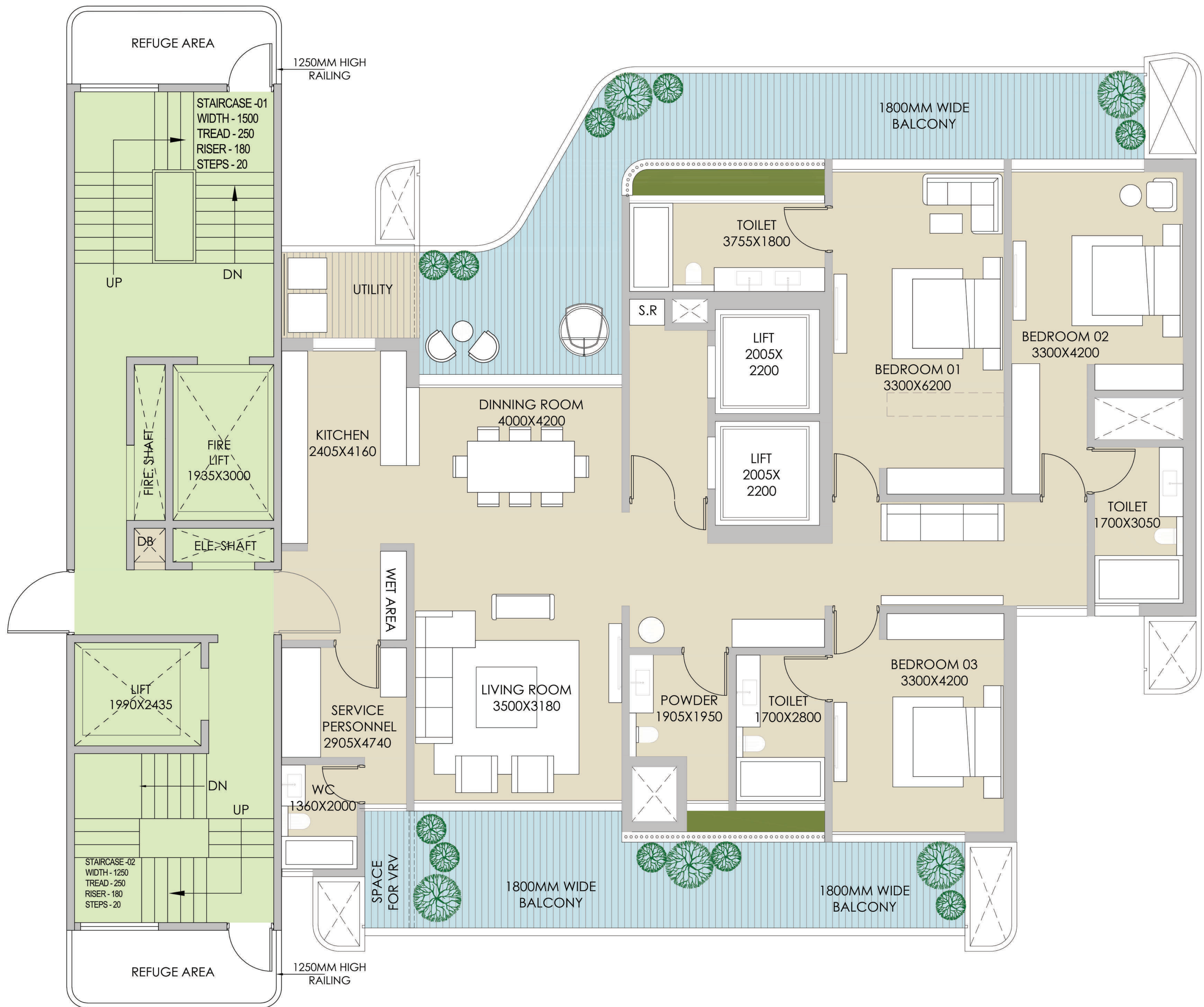
TYPICAL FLOOR PLAN : 3 BHK UNIT -3B
